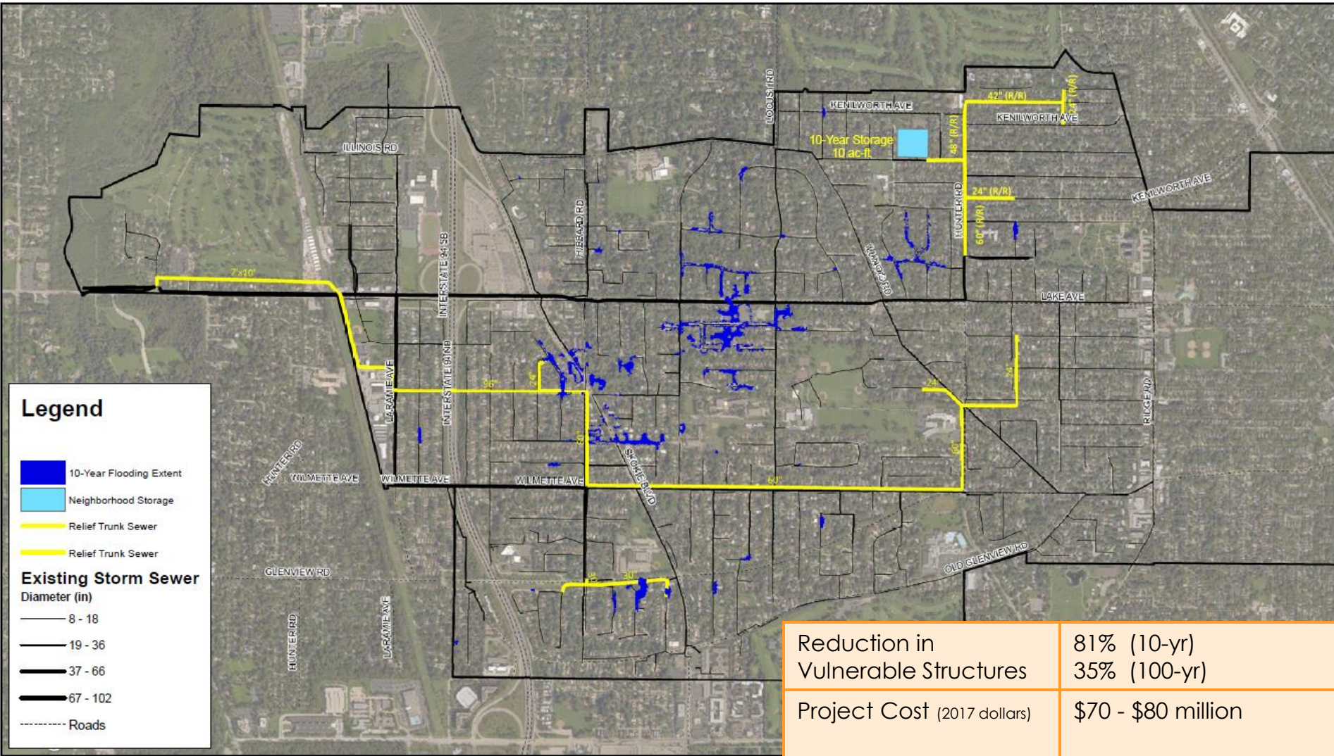
Reduced Relief Sewer Plus Neighborhood Storage Supplemental Storm Sewer Analysis Village of Wilmette
