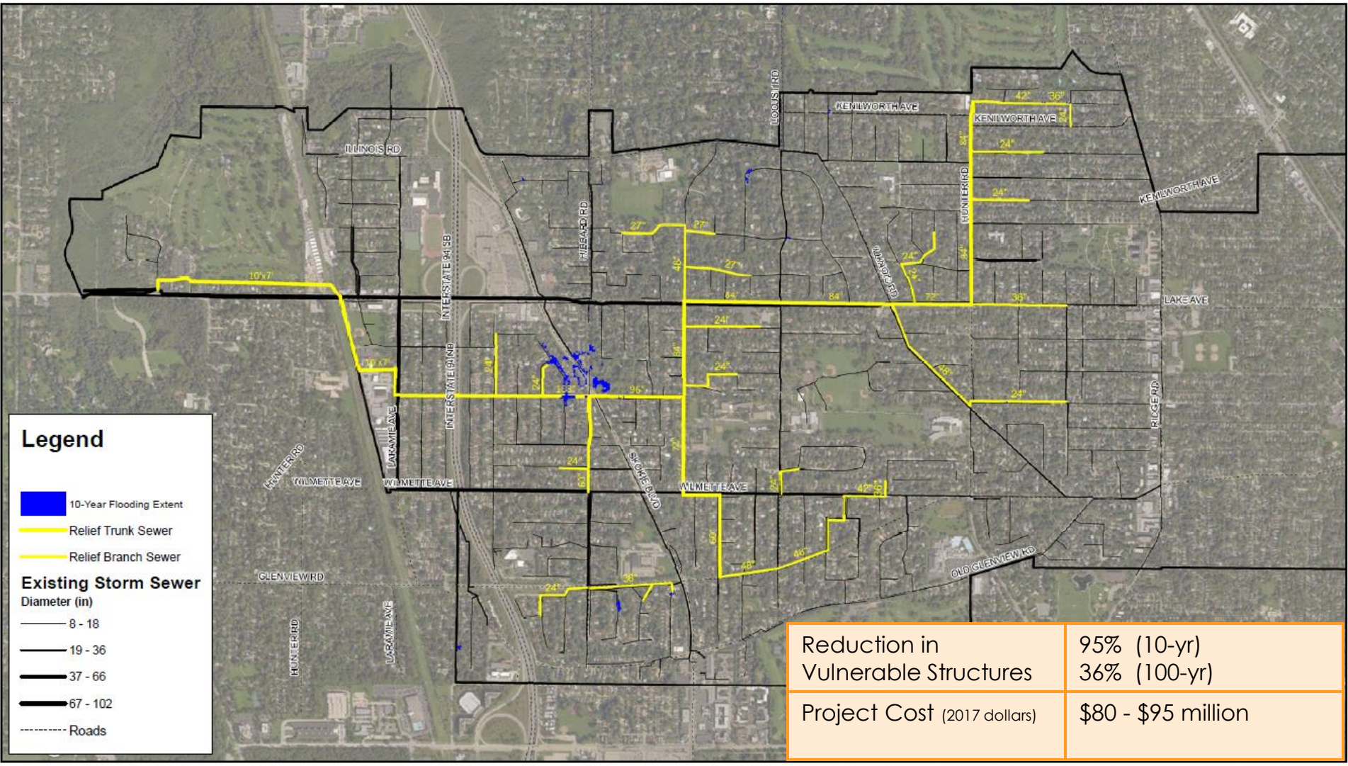
Relief Sewer Option (CBBEL Alt. 1) Supplemental Storm Sewer Village of Wilmette
